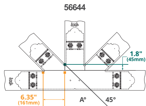
Shown From Back Viewpoint
